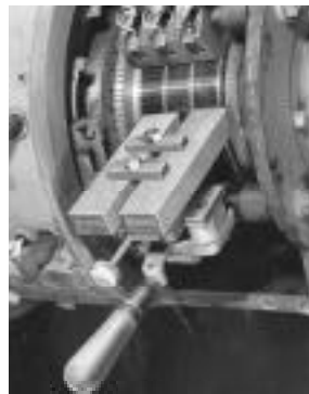
Type C mounted on Auxilliary Generator using only lower part of adjustable support.
